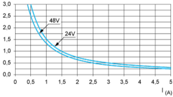
DC12 curves
